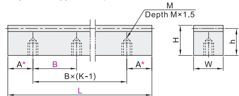
ZB (Bottom Tapped Holes)
