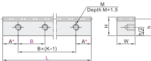
ZC (Side Tapped Holes)
