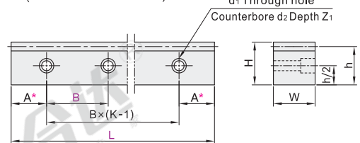
ZD (Side Counterbore Holes)
