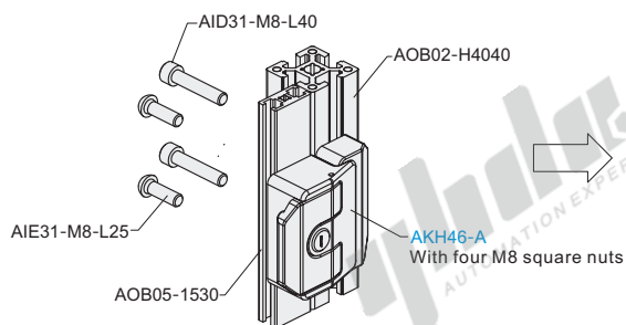
Exploded drawing
