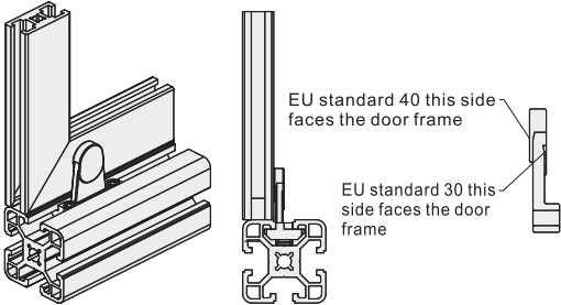
Exploded drawing
