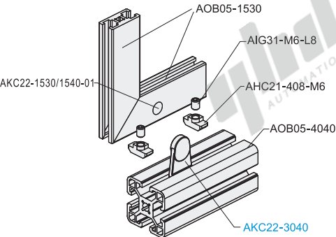
Assembly drawing
