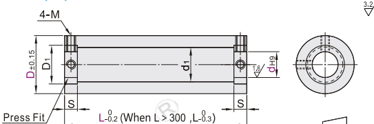
Set Screw Type QAP01/21/41
