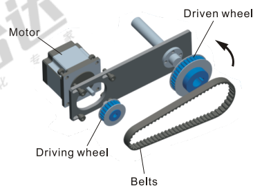
Exploded Drawing
