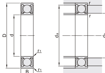
Installation Diagram
