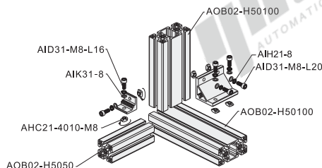
Exploded drawing
