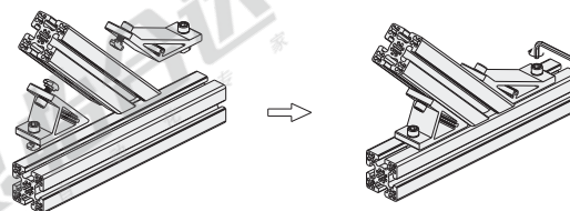
Assembly drawing
