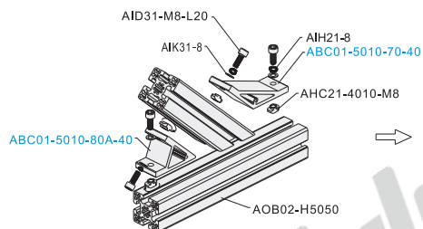
Exploded drawing
