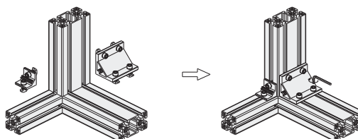
Assembly drawing
