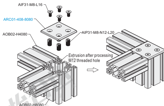
Exploded drawing
