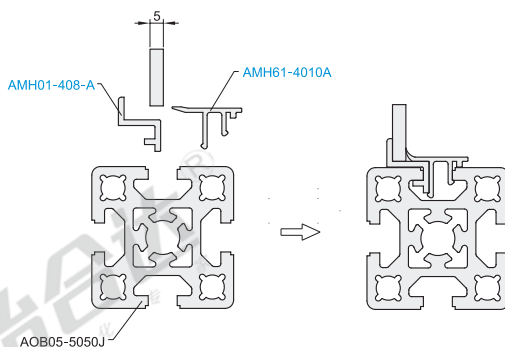
Exploded drawing
