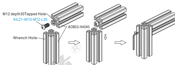
Exploded drawing
