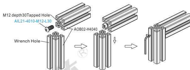
Exploded drawing
