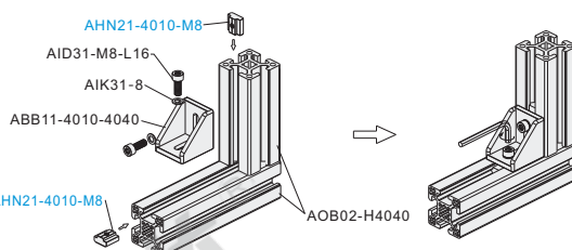
Exploded drawing
