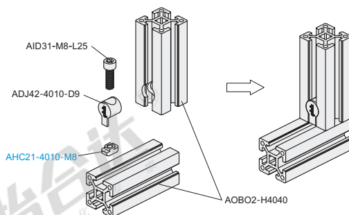
Exploded drawing
