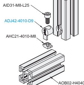
Exploded drawing
