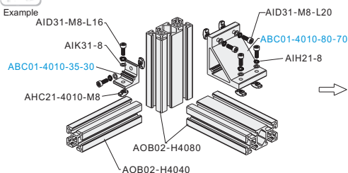
Exploded drawing
