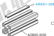
Exploded drawing
