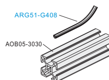
Exploded drawing
