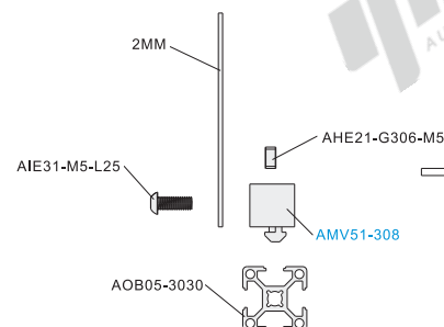
Exploded drawing
