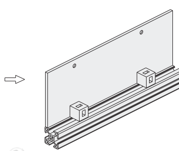
Assembly drawing
