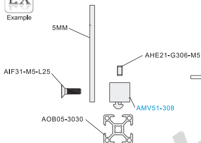
Exploded drawing
