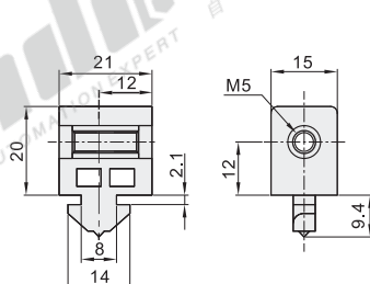
AMV53-308
