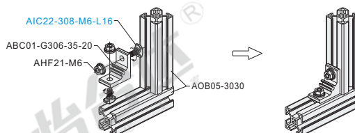
Exploded drawing
