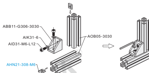
Exploded drawing
