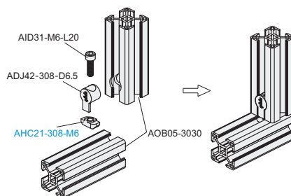
Exploded drawing
