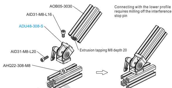
Exploded drawing
