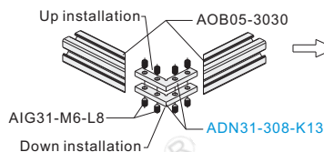
Exploded drawing
