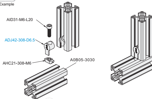
Exploded drawing
