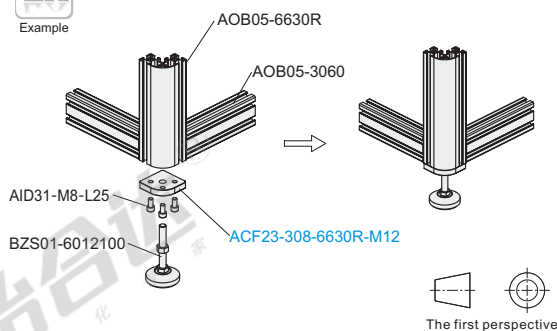
Exploded drawing
