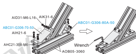
Exploded drawing
