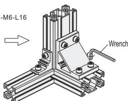
Assembly drawing
