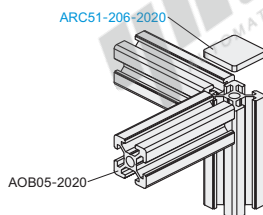
Exploded Drawing
