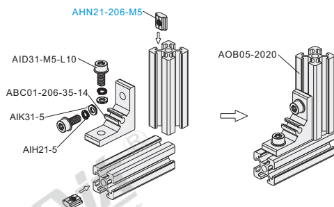
Exploded Drawing
