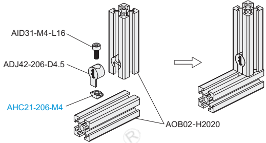
Exploded drawing
