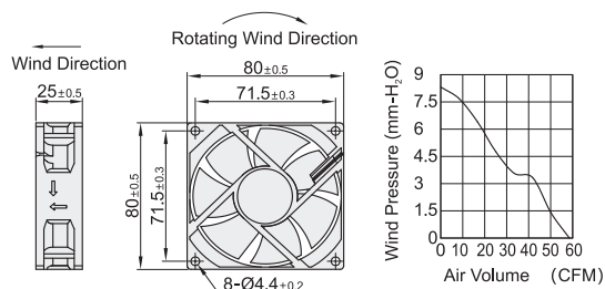
Dimensions: 8025M1
