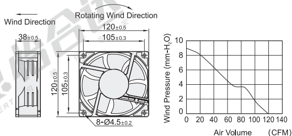
Dimensions: 12038M1/12038M3
