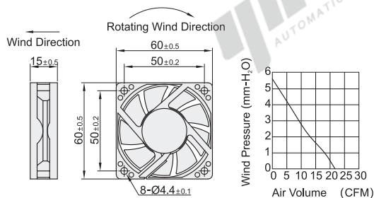
Dimensions: 6015M1
