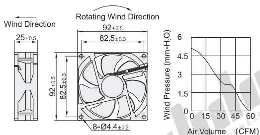
Dimensions: 9225M1
