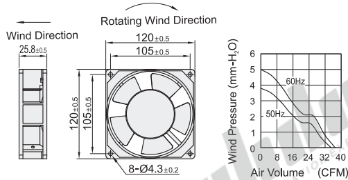
Dimensions: 120B
