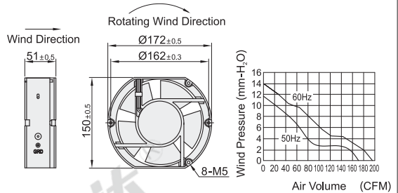
Dimensions: 172
