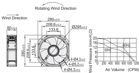
Dimensions: 280
