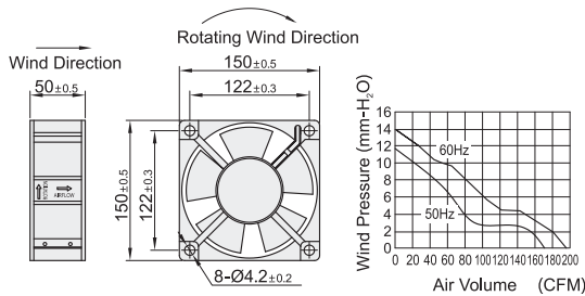
Dimensions: 150
