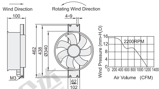
Dimensions: 340
