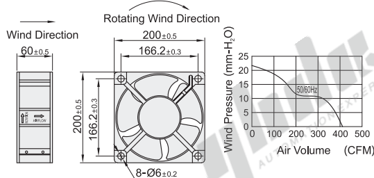
Dimensions: 200
