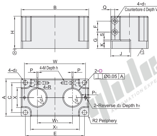
Two-Hole Base ZCD18
