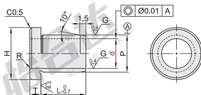
with shoulder, Thin wall Type YKY41/42/62
