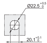
□ Cut Out Dimensions
