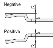
□ Lock bolt shape
