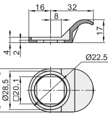
Handle Pull
