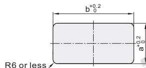
Cut Out Dimensions
