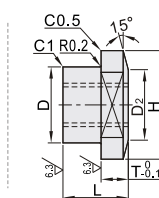
Cylinder Connector
