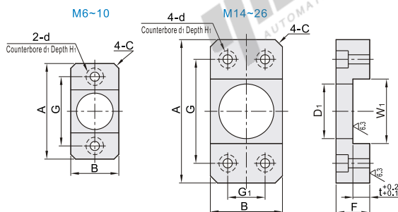
Mount Flange
