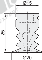
Pad Diameter \varnothing 20
