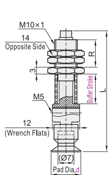
Pad Diameter Ø6~9
