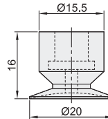
Pad Diameter Ø20
