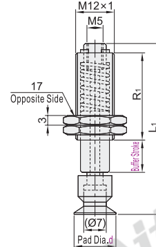
Pad Diameter Ø6~9
