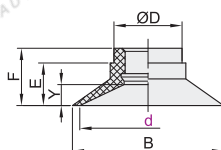
Flat Type Pad Diameter \varnothing 10 \sim 25
