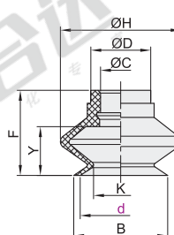
Organ Type Pad Diameter \varnothing 10 \sim 25
