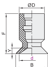
Flat Type Pad Diameter \varnothing 2 \sim 8
