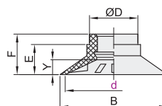
Flat Type with Ribs Pad Diameter \varnothing 10 \sim 25
