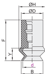
Organ Type Pad Diameter \varnothing 6 \sim 8
