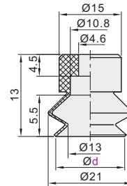
Pad Diameter \varnothing 20
