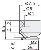
Pad Diameter Ø6
