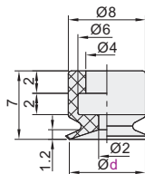
Pad Diameter Ø8
