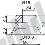
Pad Diameter Ø20
