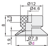
Pad Diameter Ø15
