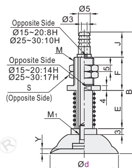
Pad Diameter Ø15~30
