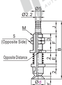
Pad Diameter Ø5~8
