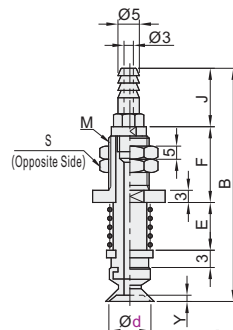
Pad Diameter Ø10
