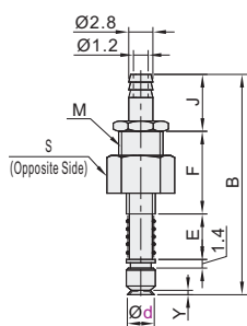
Pad Diameter Ø2, 3.5
