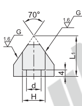
Lower Part
