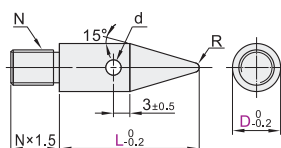
Taper R PAJ61 PAJ66
