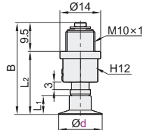
Spring Type, Direct-Mount J-WEU76/77
