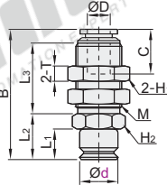
Pad Diameter Ø10
