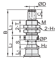
Pad Diameter Ø15~30
