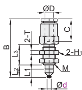
Pad Diameter Ø4
