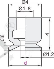
Pad Diameter \varnothing 4
