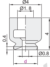
Pad Diameter \varnothing 3
