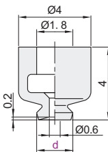
Pad Diameter \varnothing 2
