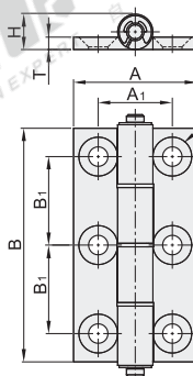
6 Holes Installation
