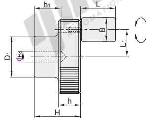
Round Hole HBA01 HBA02
