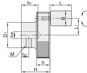
Hole + Tap HBA11 HBA12 HBA16
