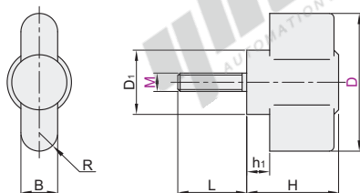
Threaded HAQ11
