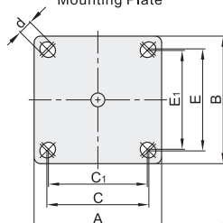
CLB06-D50/65/75 Mounting Plate
