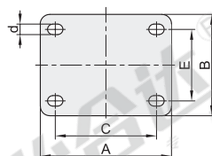
CLD06-D65A/D75A Mounting Plate
