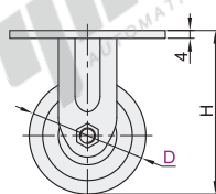
CLB06-D50/65/75 Mounting Plate
