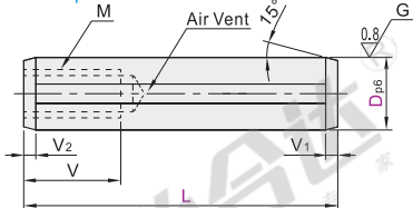
Air Vent, Tolerance p6 BLV71-p6
